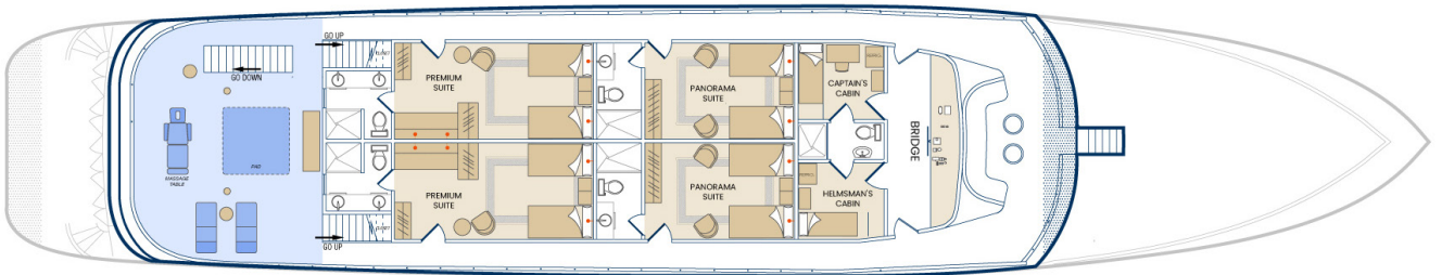
BRIDGE DECK
