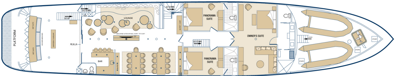
MAIN DECK
