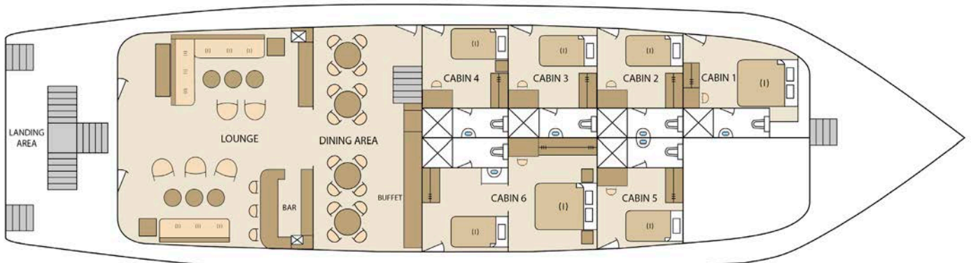
MAIN DECK
